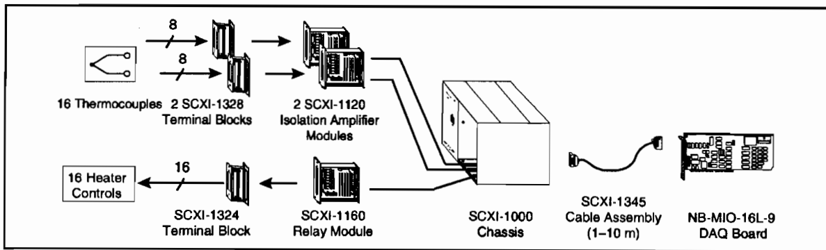
Figure 8. SCXI Temperature Control System
