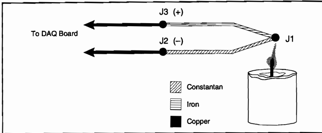
Figure 2. J-Type Thermocouple
